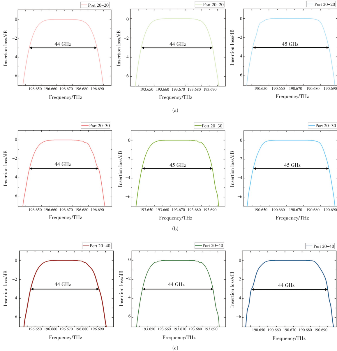
▲ Figure 10. Bandwidth performance at 50 GHz grid with the center wavelengths of 1 524 nm, 1 548 nm, and 1 572 nm from left to right for the deflections from port 20 to 20, 30, and 40, respectively
