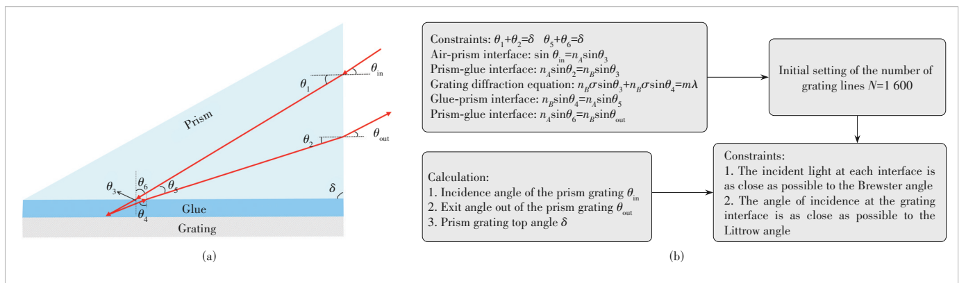
▲ Figure 4. Schematic diagram of (a) prism grating and (b) its design process
