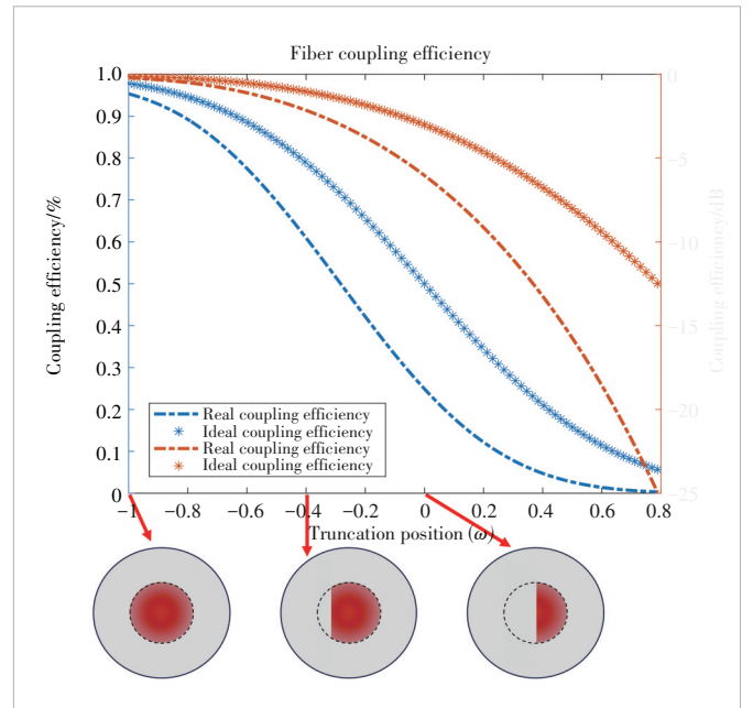
▲ Figure 6. Fiber coupling efficiency for different truncation ratios
