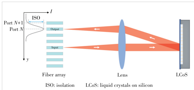
▲Figure 7. Port isolation of a WSS system
