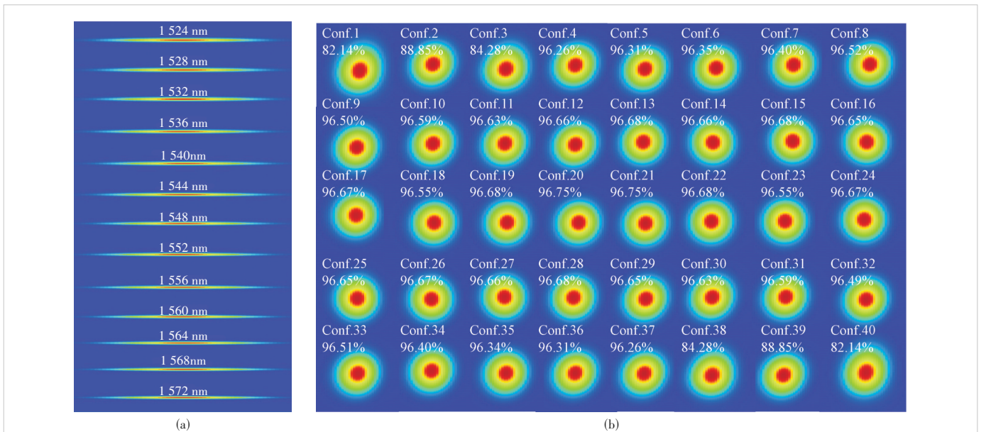
▲ Figure 9. Deflection performance of the WSS system in Zemax: (a) layout of Gaussian beams on the LCoS and (b) shape of the beam to be coupled into the fiber
