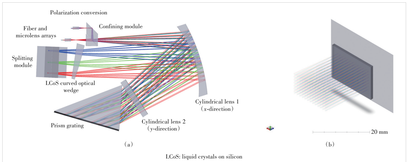
▲ Figure 8. Schematic diagram of the optical structure of WSS in Zemax: (a) overall component layout and (b) model of LCoS
