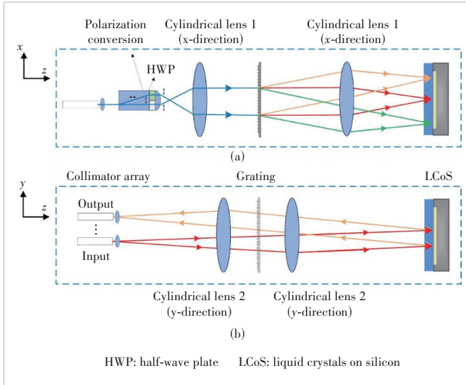
▲ Figure 2. Optical paths of WSS in (a) the dispersion direction and (b) the switching direction
