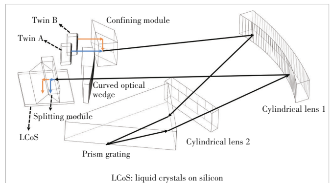
▲ Figure 1. Twin WSS architecture
