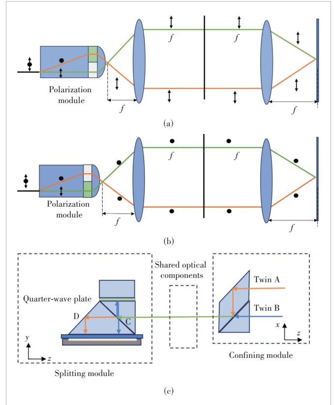
▲ Figure 3. Schematic illustration of symmetric polarization loops established in the WSS: (a) polarization diversity of source A; (b) polarization diversity of source B; (c) polarization multiplexing in the twin WSS
