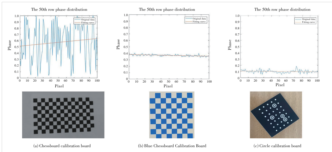
▲ Figure 2. Different calibration board's phase distribution
