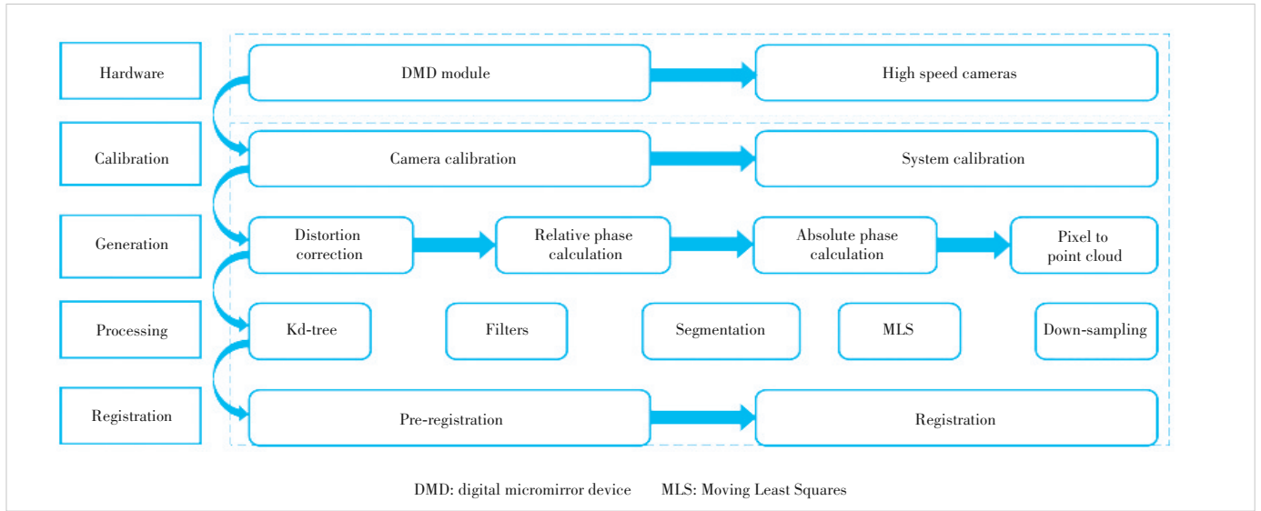
▲ Figure 1. Proposed system setup formed by hardware and software
