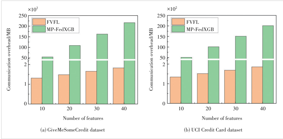
▲ Figure 2. Communication overheads for different numbers of features ( F )
