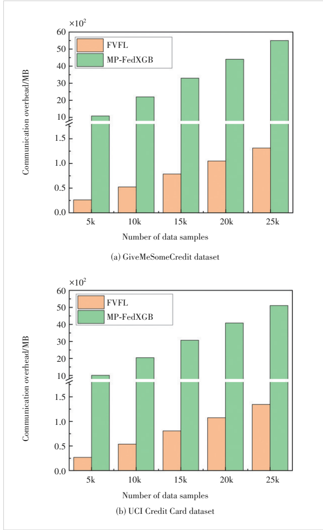
▲ Figure 5. Communication overheads for different numbers of data samples ( I )
