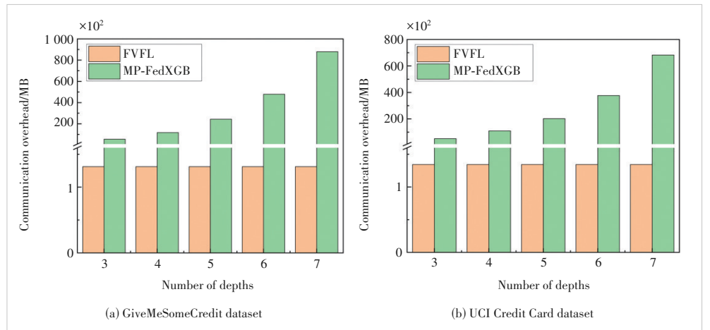
▲ Figure 4. Communication overheads for different numbers of depths ( D )
