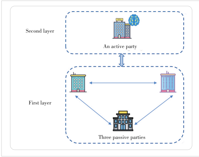
▲ Figure 1. Architecture of the proposed FVFL framework
