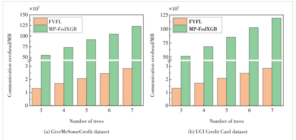
▲ Figure 3. Communication overheads for different numbers of trees ( T )
