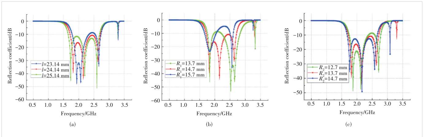
Figure 3. Simulation scattering parameter results of FSS unit cell: (a) results with different cross slot lengths l ; (b) results with different top patch radii R_1 ; (c) results with different middle patch radii R_2
